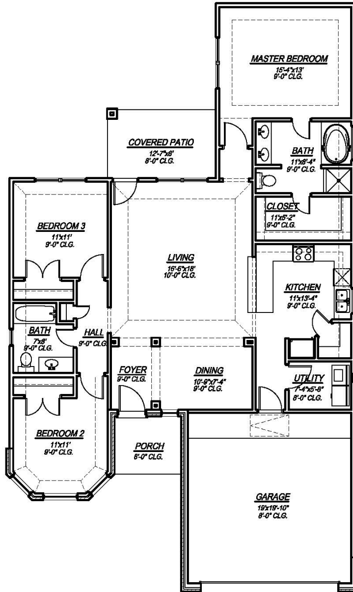
Floor Plan B
